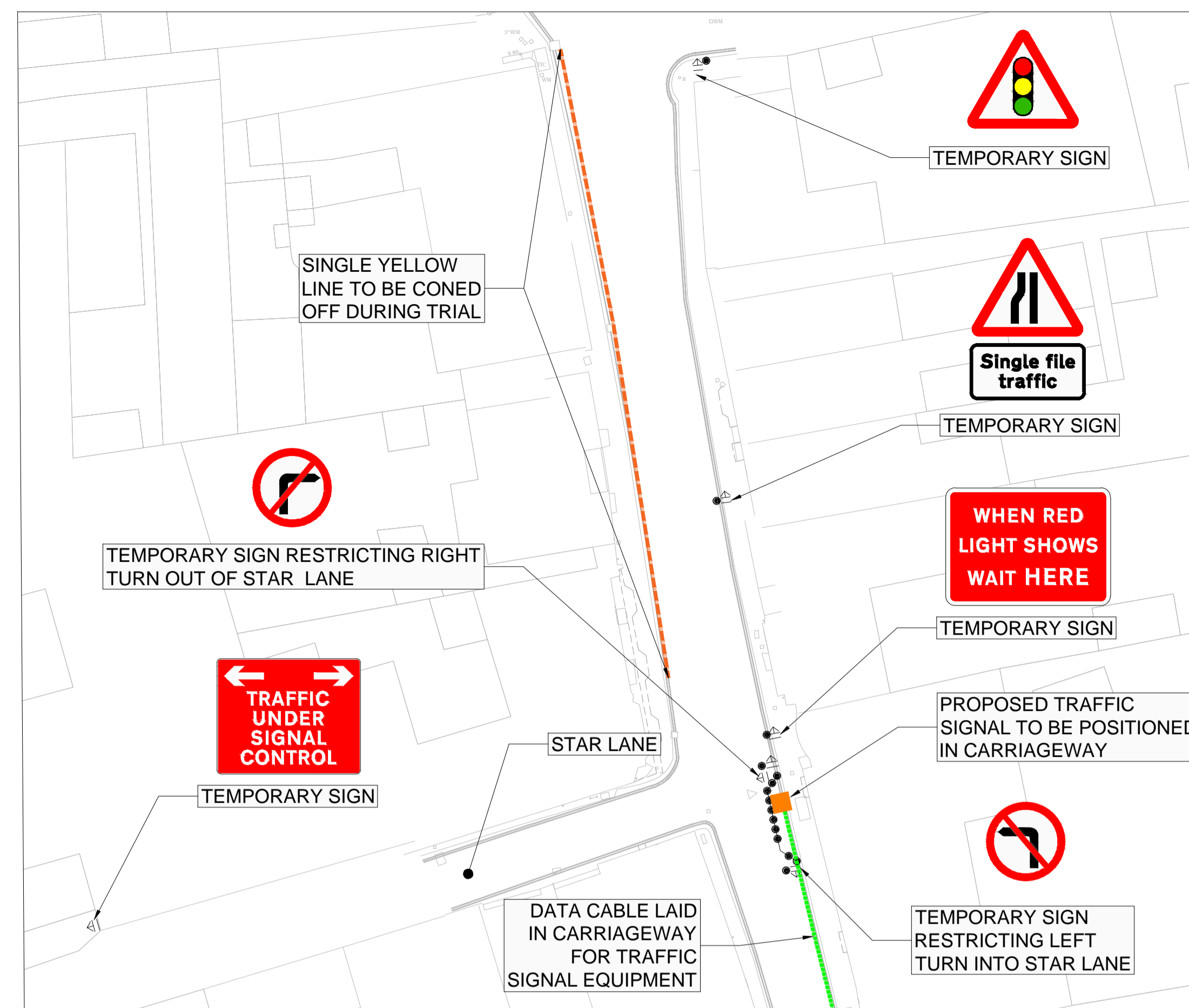
Temporary Traffic Signal Layout at Star Lane Junction
